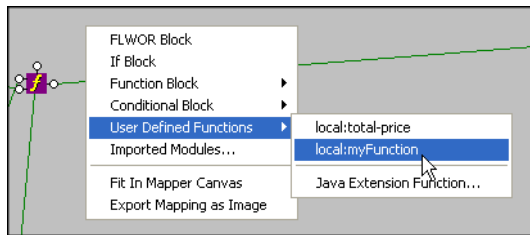
Figure 355. User-Defined Functions
