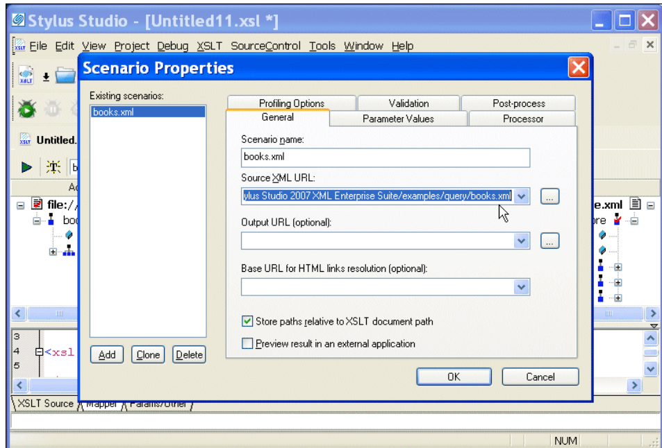
Figure 258. XSLT Scenario
