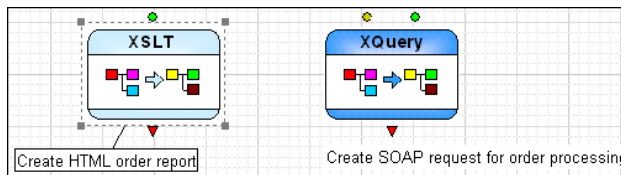
Figure 496. Pipeline Labels
