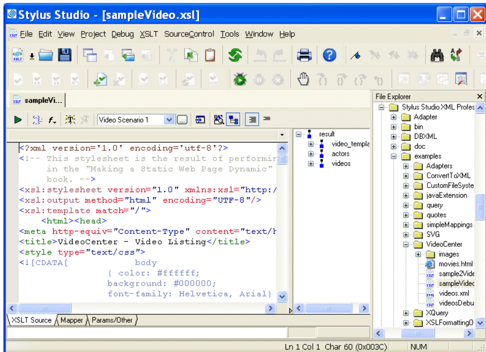
Figure 238. XSLT Editor
