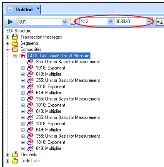
Figure 211. Full Specification
